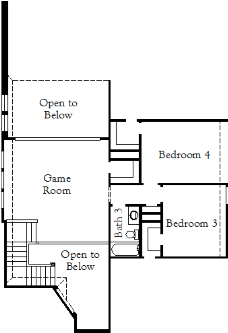
Second Floor
