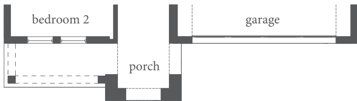
FIRST FLOOR - ELEVATION D
