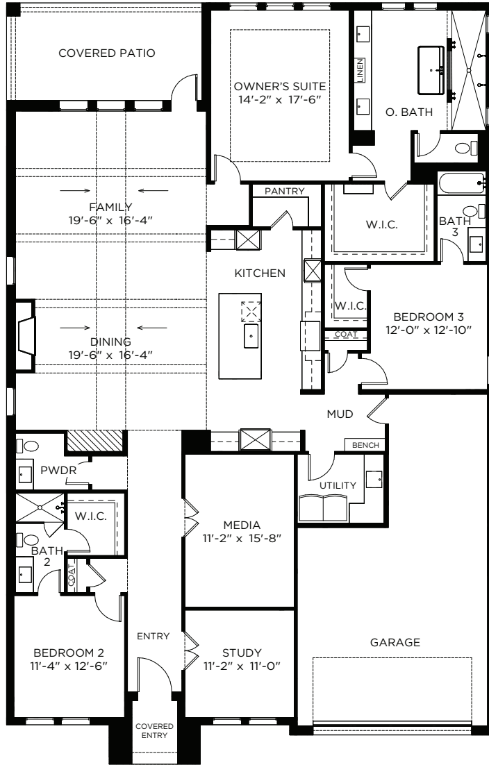
1ST FLOOR PLAN - ELEVATION A*
