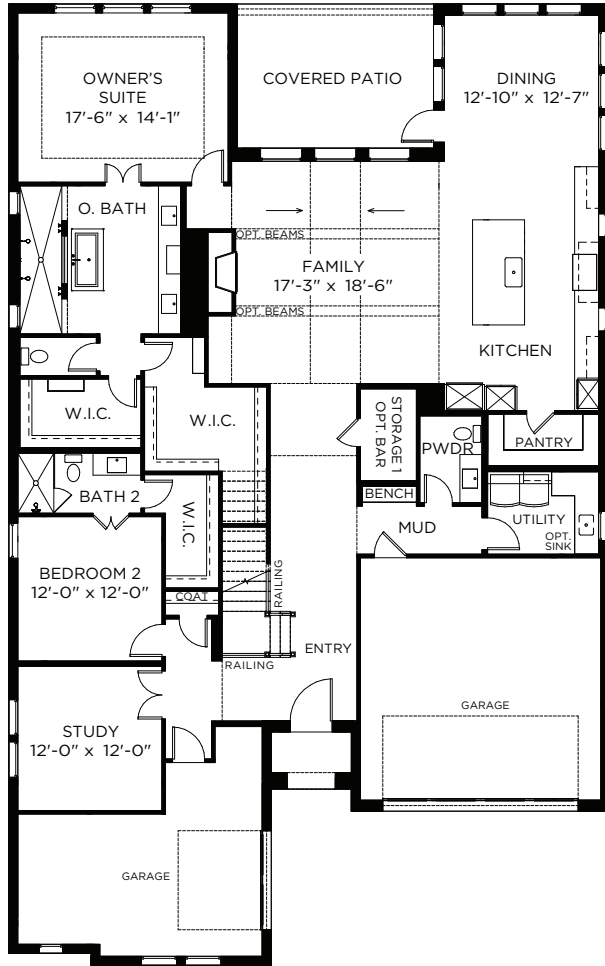
1ST FLOOR - ELEVATION A*
